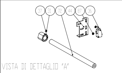
Impastatrice a spirale TSVX60 (vasca estraibile) - Spiral dough mixer TSVX-60 (extractable bowl)
