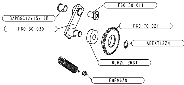
DETAIL A ECHELLE 1:5
